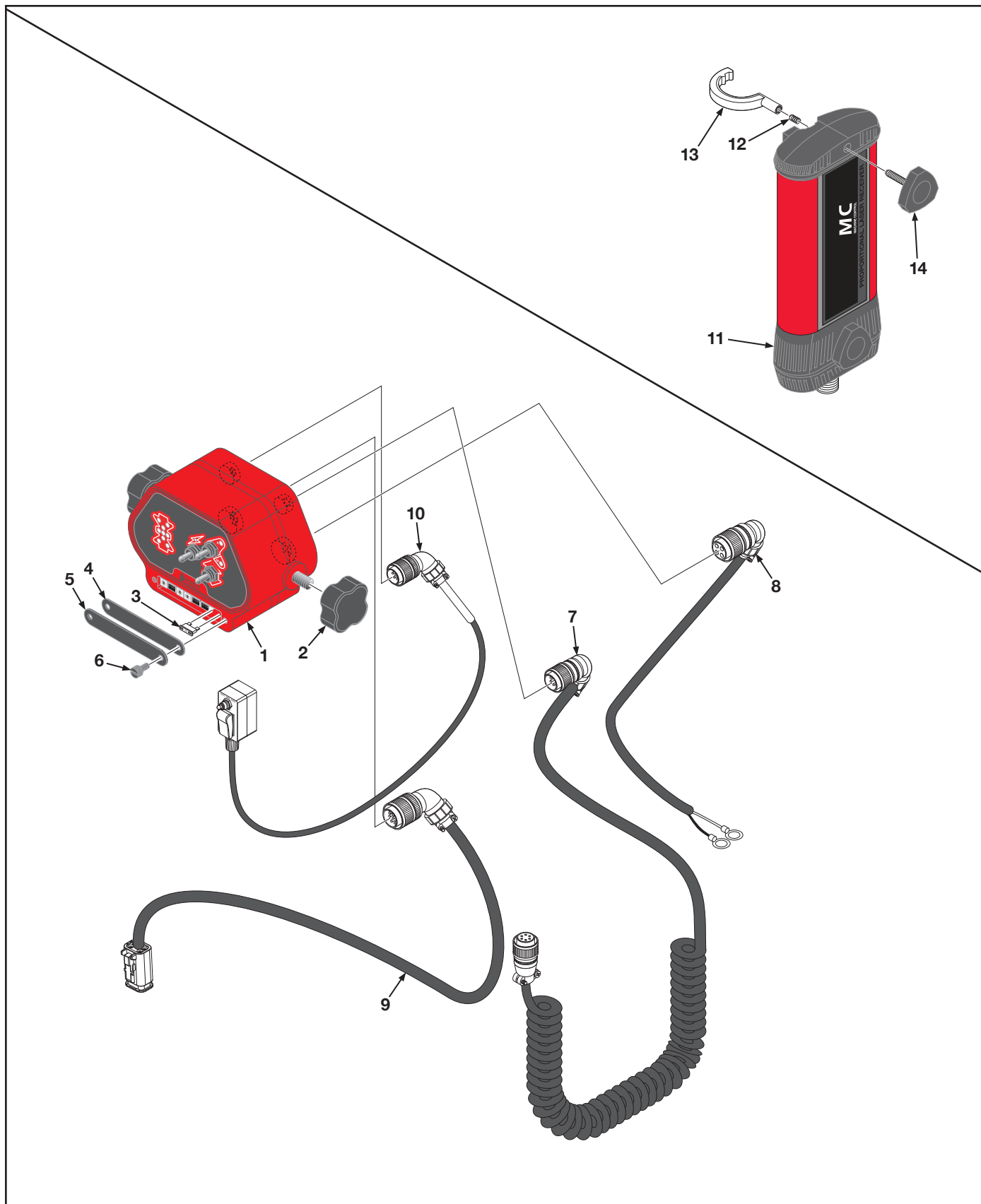
Figure 6. Control Panel, Laser Receiver 360°, Cables - Apache CB26/Spectra CB25
