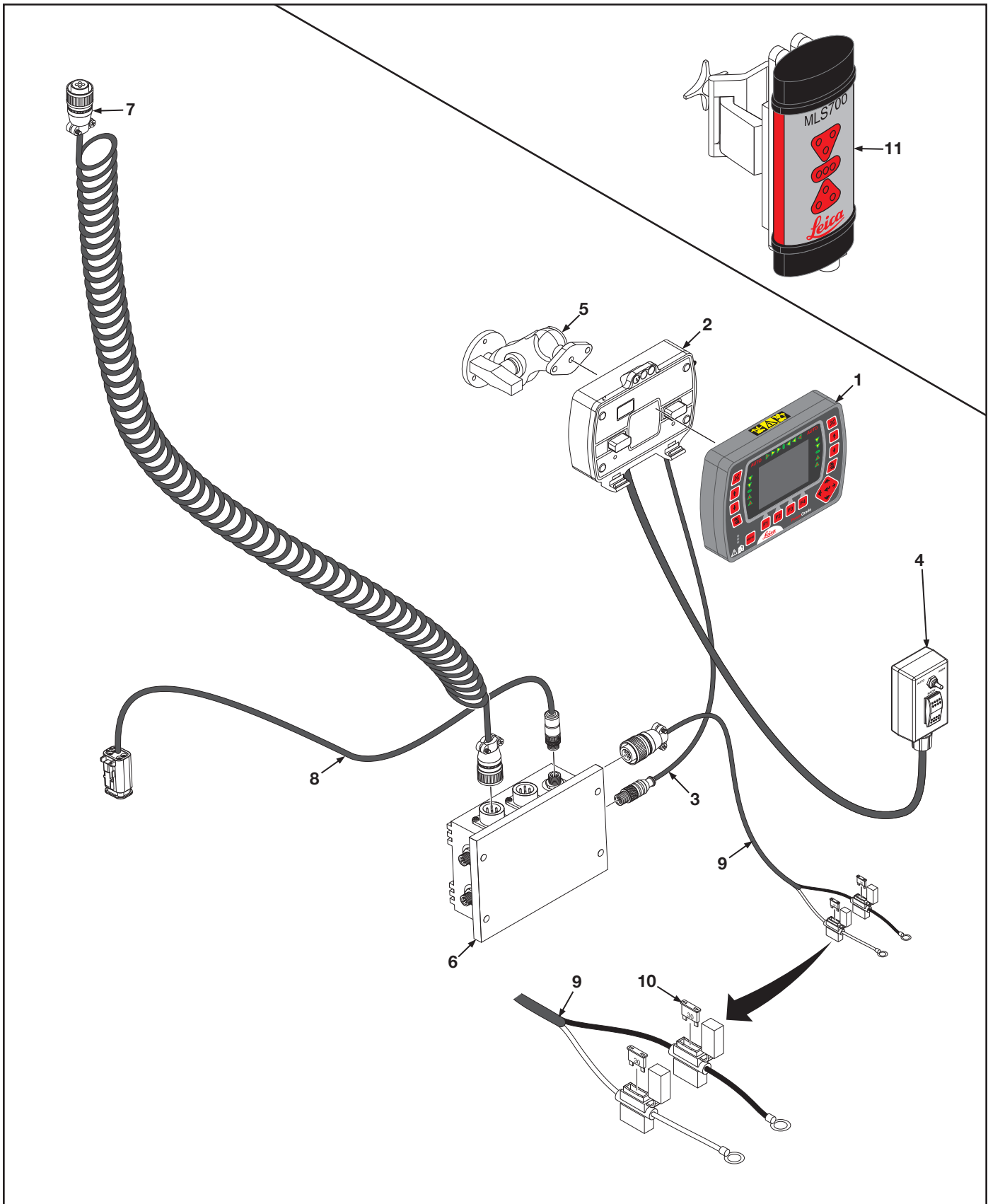
Figure 8. Control Panel, Laser Receiver 360°, Cables - Leica MCP-1300
